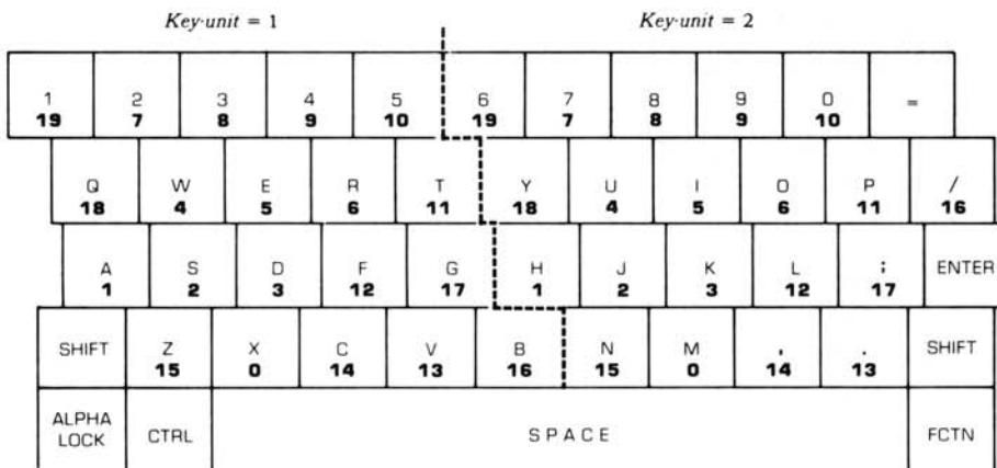
Figure 1. Split Keyboard Scan. Codes returned = 0 through 19.
